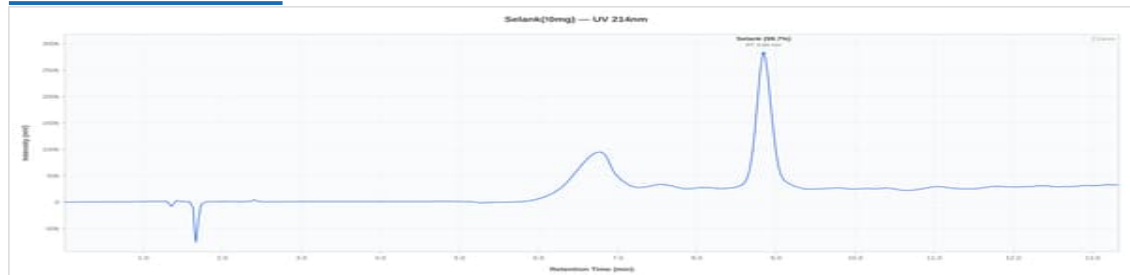
Selank 10 - 062126: UV Chromatogram
